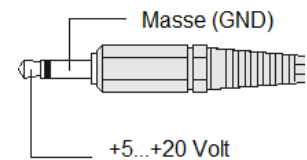
Connector assignment (3.5 mm barrel plug)
