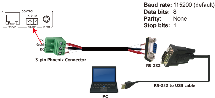
Figure 1: 3-pin phoenix connector to USB
