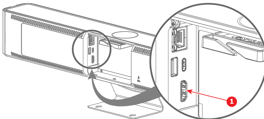
Image 4–12 Where to connect the HDMI cable
