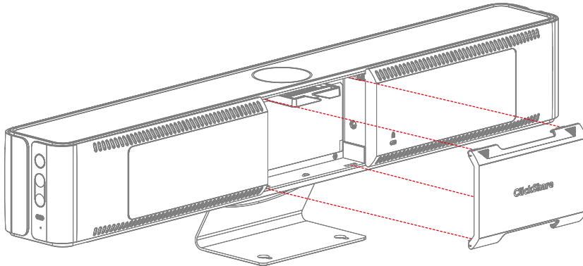
Image 4–14 Cable cover removal
