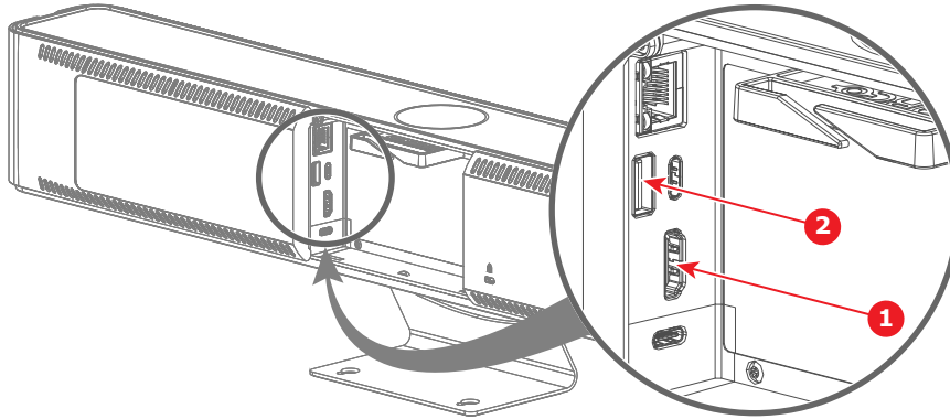
Image 4–13 Where to connect both the HDMI cable and the USB-A cable (only for touch screen)
