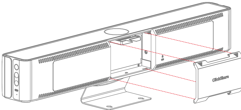
Image 4-6 Cable cover removal
