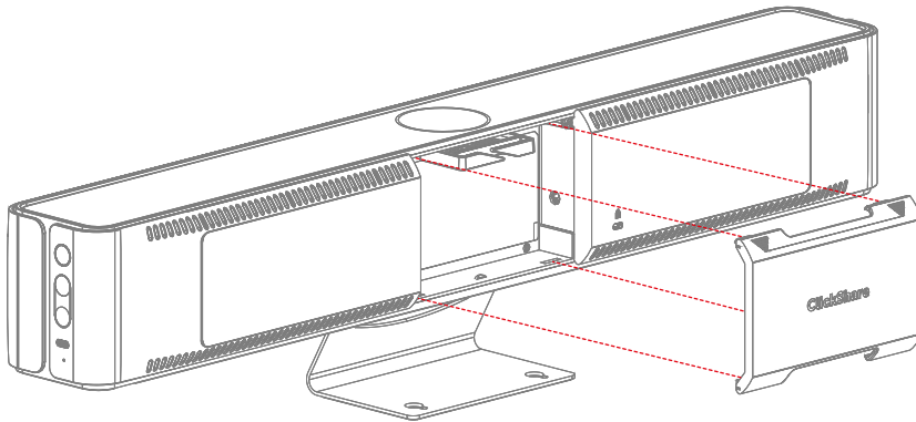
Image 4–11 Cable cover removal
