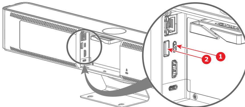
Image 4–16 Where to connect the USB-C cable or dongle and the USB-A cable (only for touch screens)
